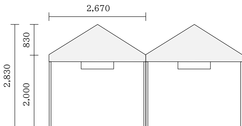
◎立面図(PLAN③)
